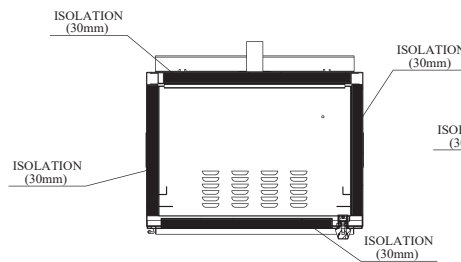
UPPER VIEW
