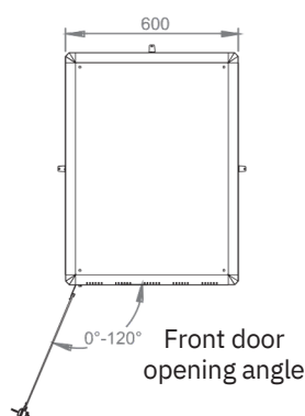
19" DYNAmic Series Free Standing Cabinets W=600 mm D=800 mm
