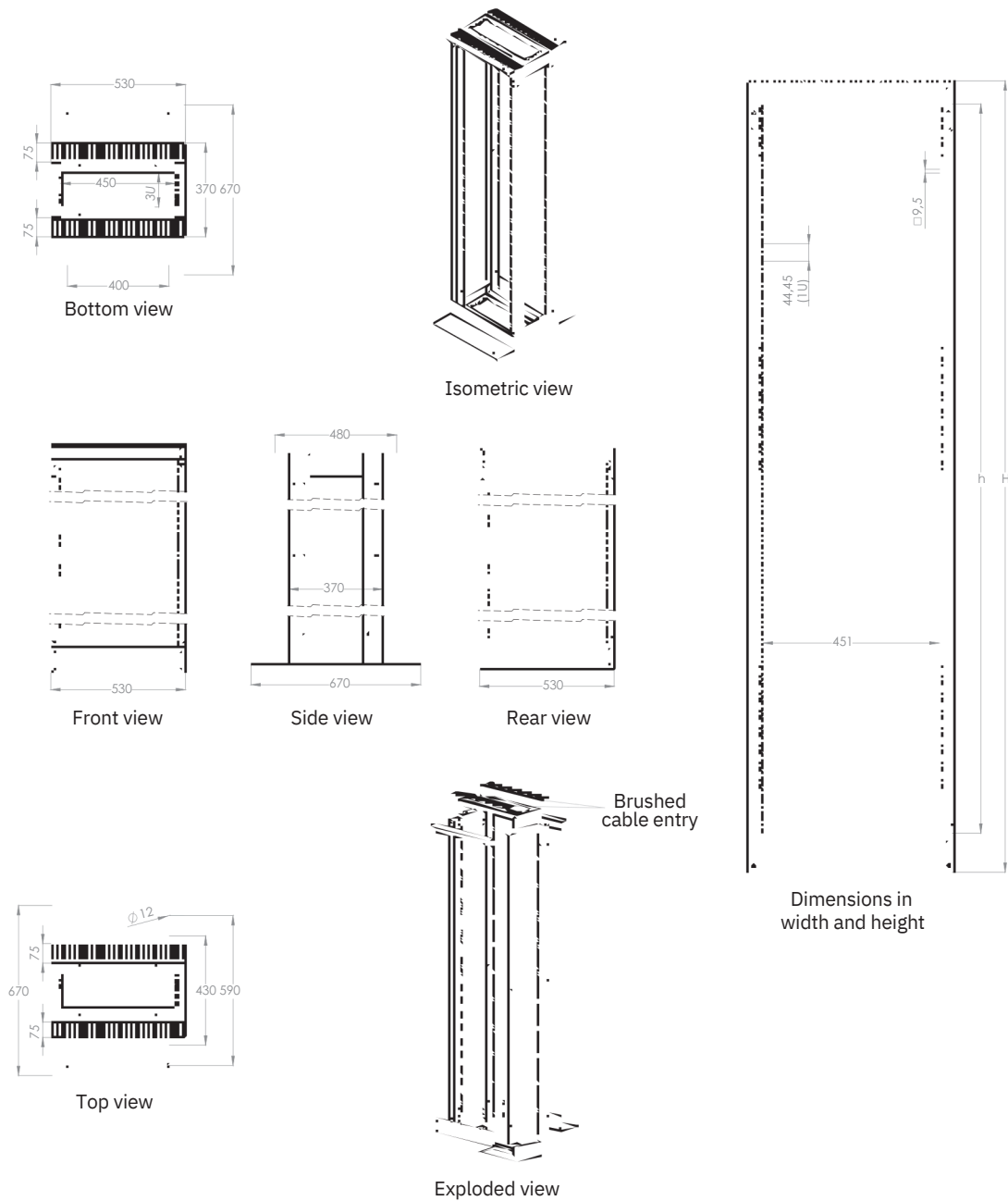
19'' DYNAframe Open Frame System Racks Double Frames d=80 mm Frame Unit W=530 mm D=670 mm
