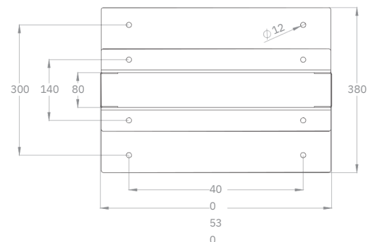
Top view mounting dimensions
