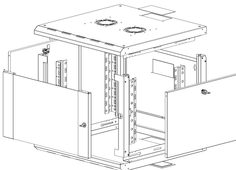
Exploded view
