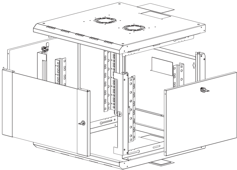
Exploded view
