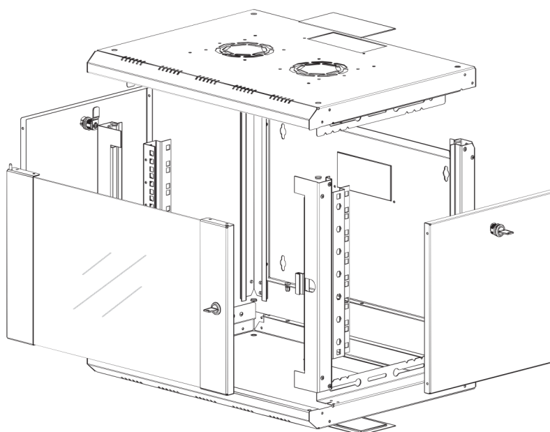
Exploded view
