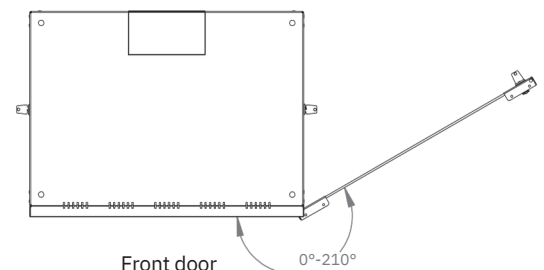
Front door opening angle
