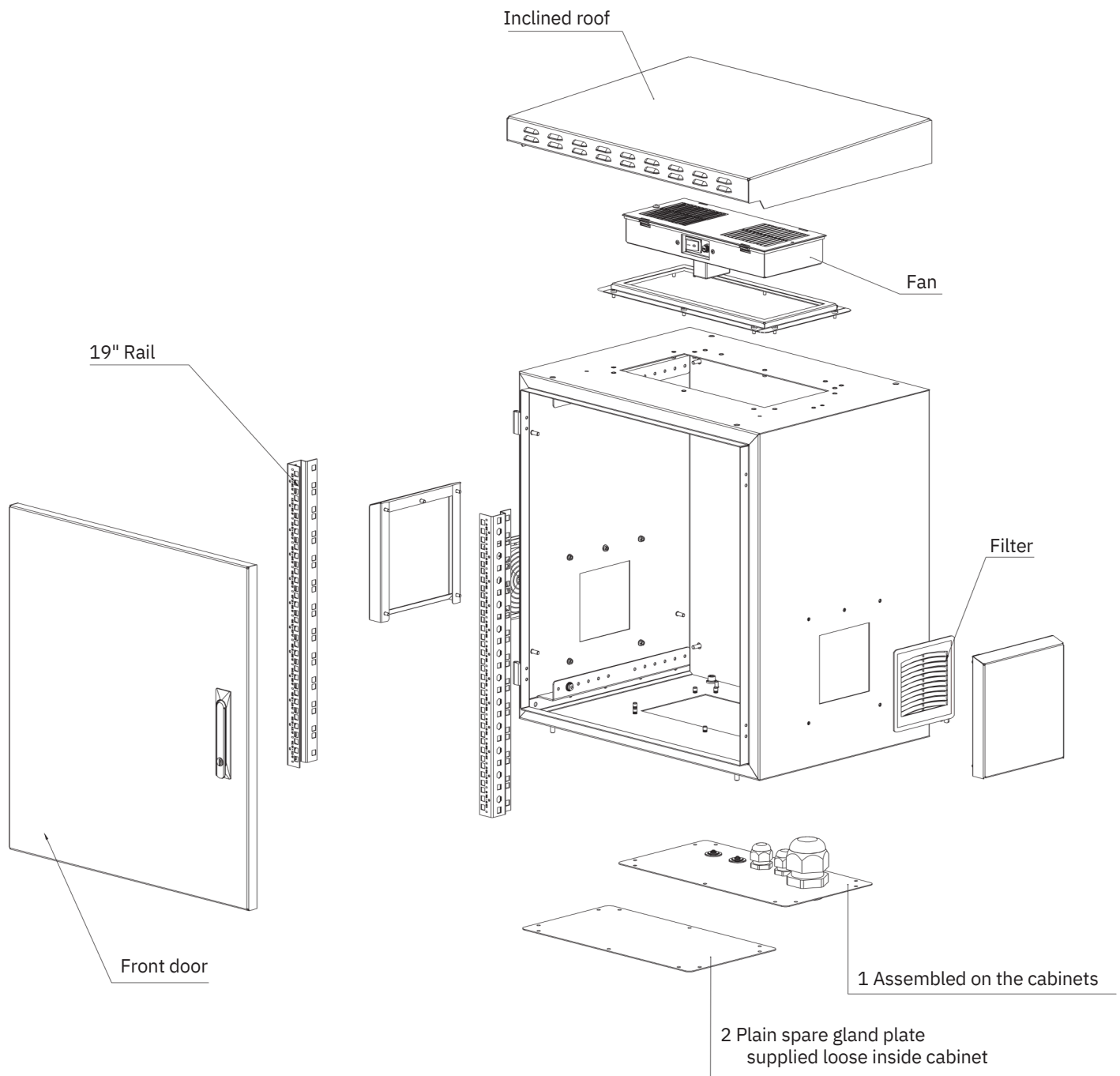
Exploded view
