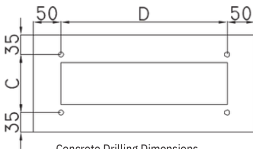
Concrete Drilling Dimensions
