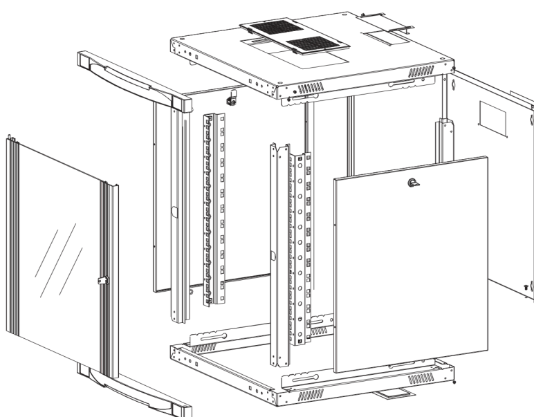
Exploded view
