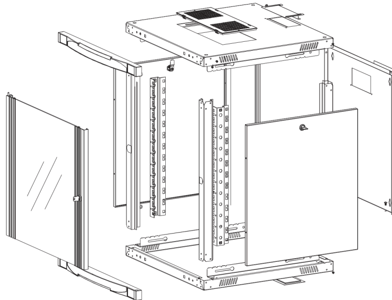
Exploded view
